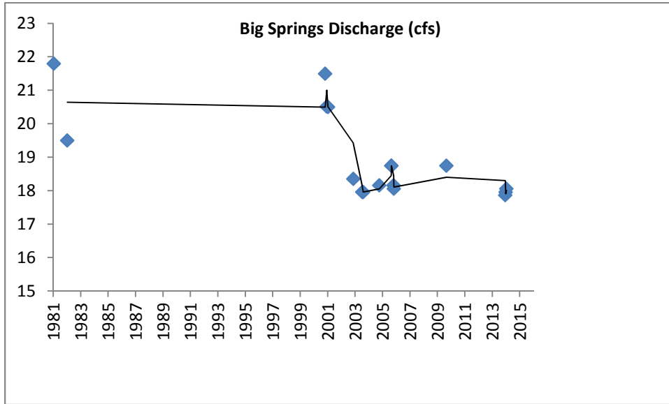
Big Springs discharge at City Park showing drop in flow between 2001 and 2003. Data in the 1980's are from USGS open file report 86-85. Measures thereafter are from Ecosystems Northwest.
